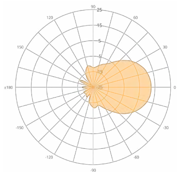
N5-X12 (12 dBi)
