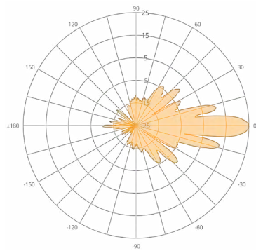
N5-X25 (25 dBi)
